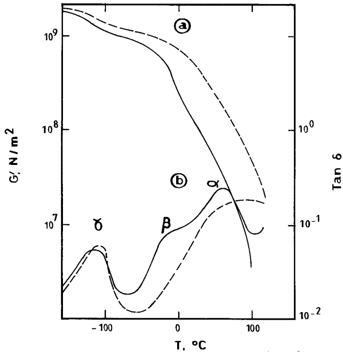
Figure 13.23 Shear modulus (a) and damping (b) at 1 Hz as a function of temperature for a branched and a linear polyethylene: (----) Ziegler polyethylene; (—) Alkathene. (From Heijboer, J., Brit. Polymer J. , 1, 3, 1969. With permission.)
