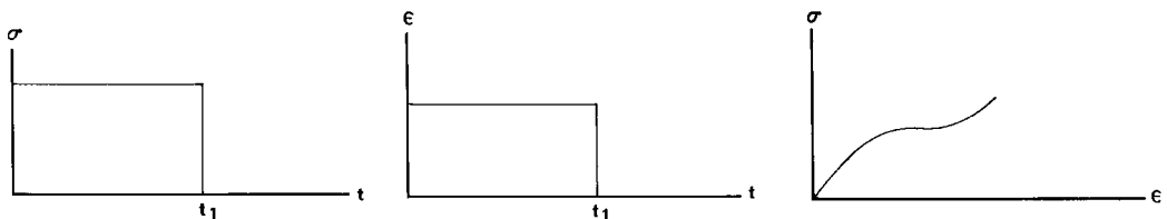
Figure 14.3 Rubber elasticity.
