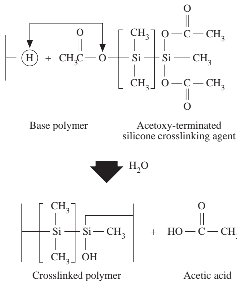
Figure 5.13 Structure of Cardiothane. (From Gogolewski, S., Colloid Polym. Sci. , 267, 757, 1989. With permission.)
